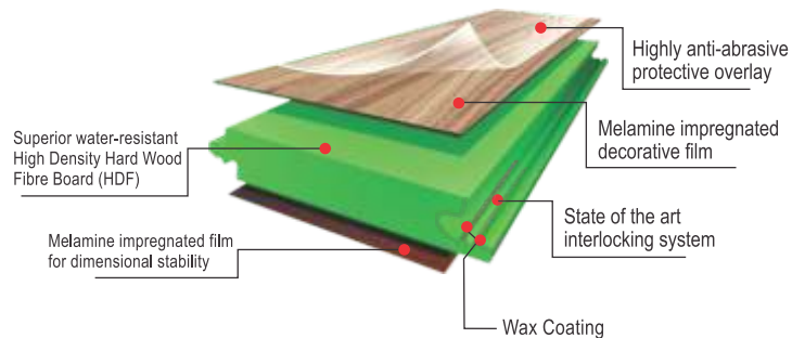
Action TESA Laminate Wooden Flooring Construction
